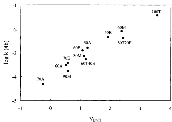
Figure 2. Correlations of \log k for 4b against Y_{\text{BnCl}} . Abbreviations for solvents as in Table 1.
