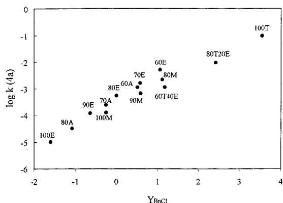
Figure 1. Correlations of \log k for 4a against Y_{\text{BnCl}} . Abbreviations for solvents as in Table 1.
