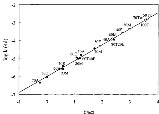
Figure 3. Correlations of \log k for 4d against Y_{\text{BnCl}} . The open circles denote the points of interpolation. Abbreviations for solvents as in Table 1.
